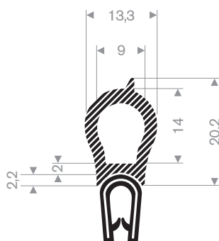
245.00.820 pvc + mosrubber klembereik 1-3 mm
